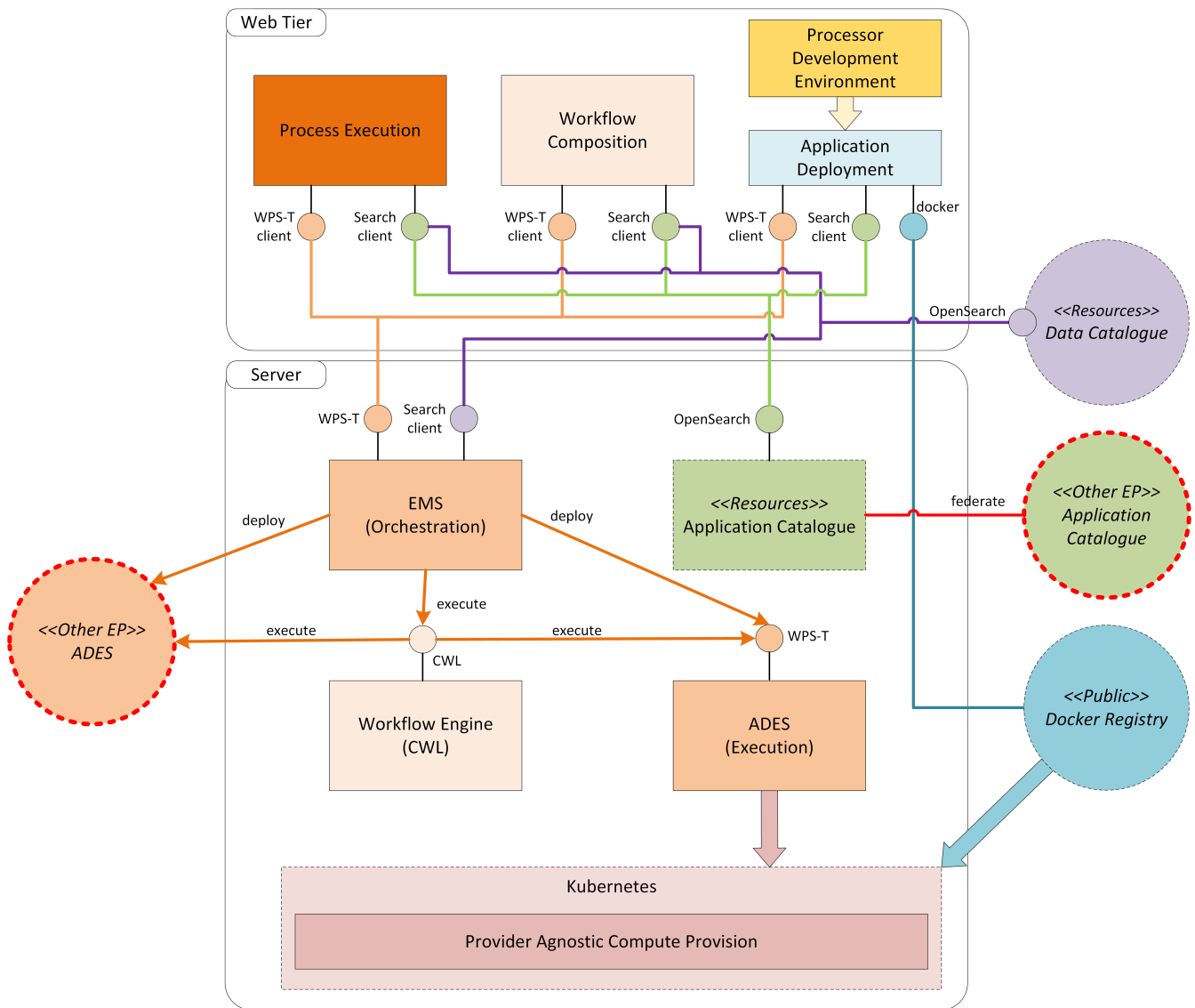
Figure 13. Processing & Chaining Overview
