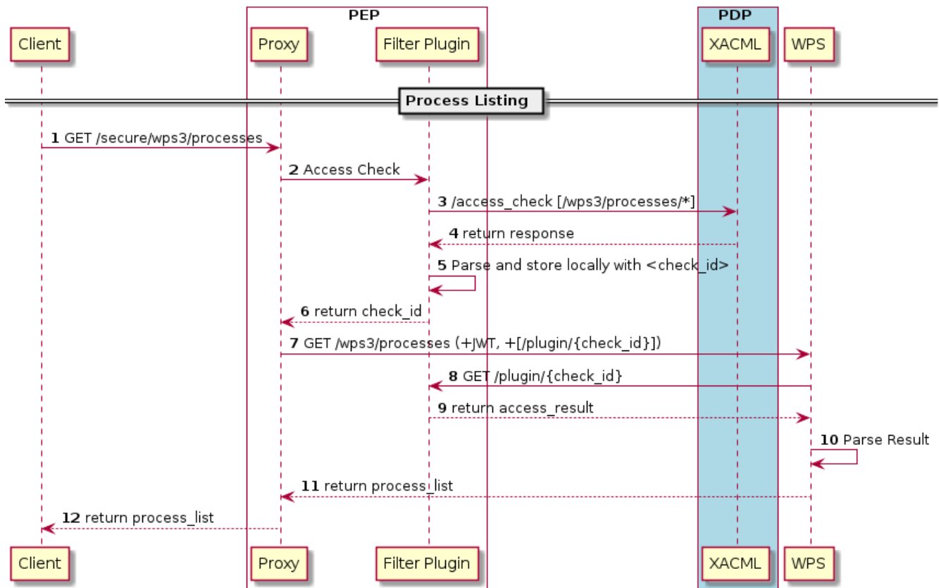
Figure 10. Policy Context Propagation through PEP protected requests.
