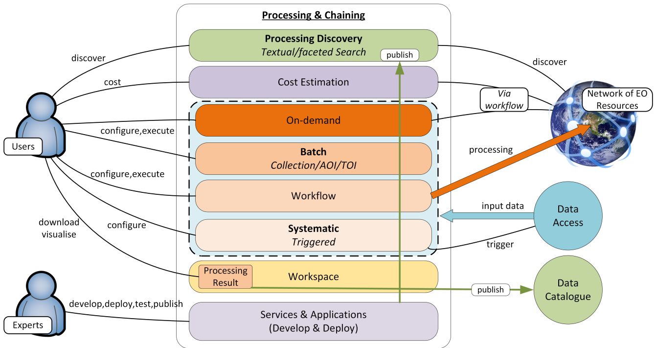
Figure 12. Processing & Chaining Use Case
