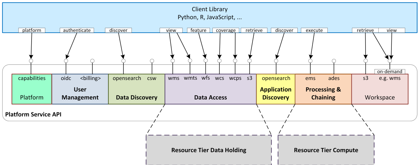
Figure 26. Client Library Service Interfaces
