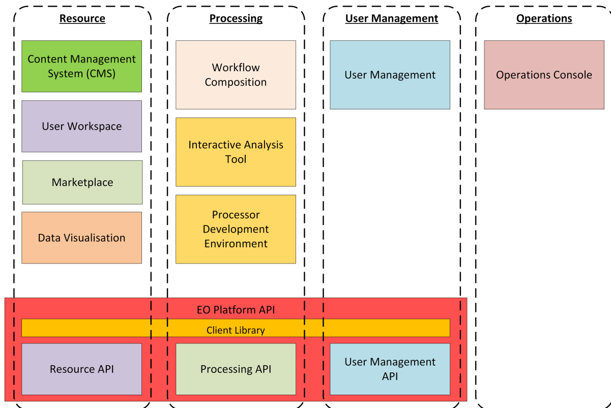
Figure 28. Web Portal: Overview
