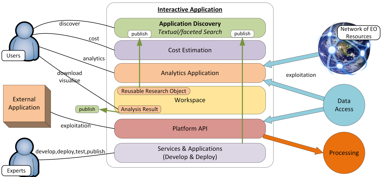
Figure 20. Interactive Applications Use Case
