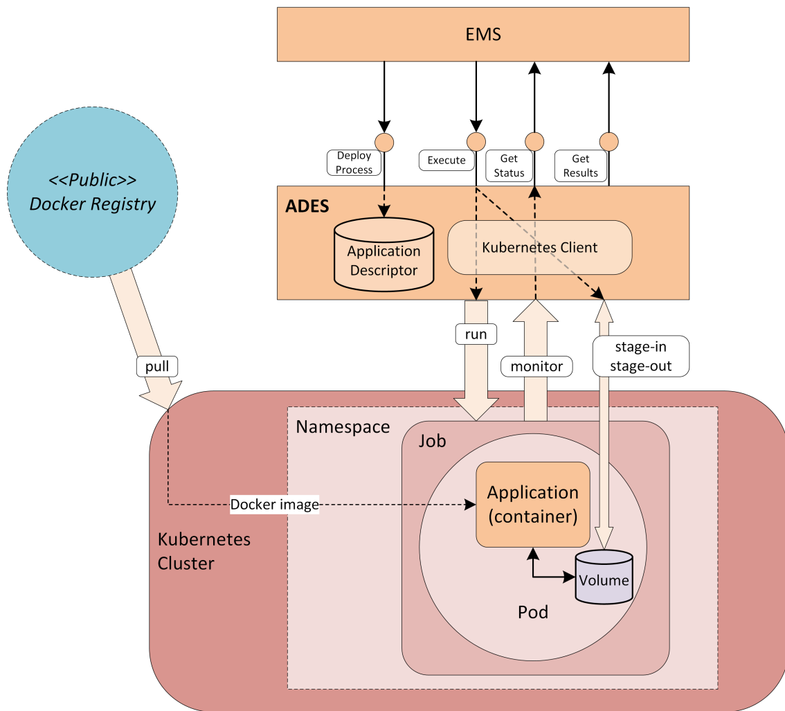
Figure 17. ADES Process Execution
