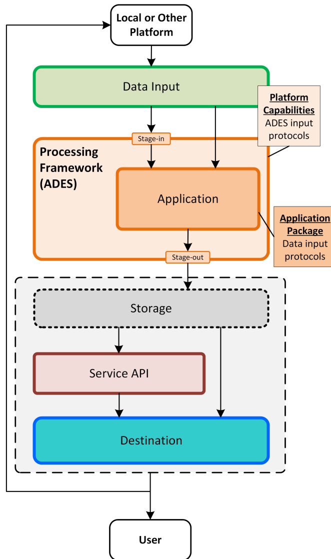
Figure 18. Processing Framework Data Access
