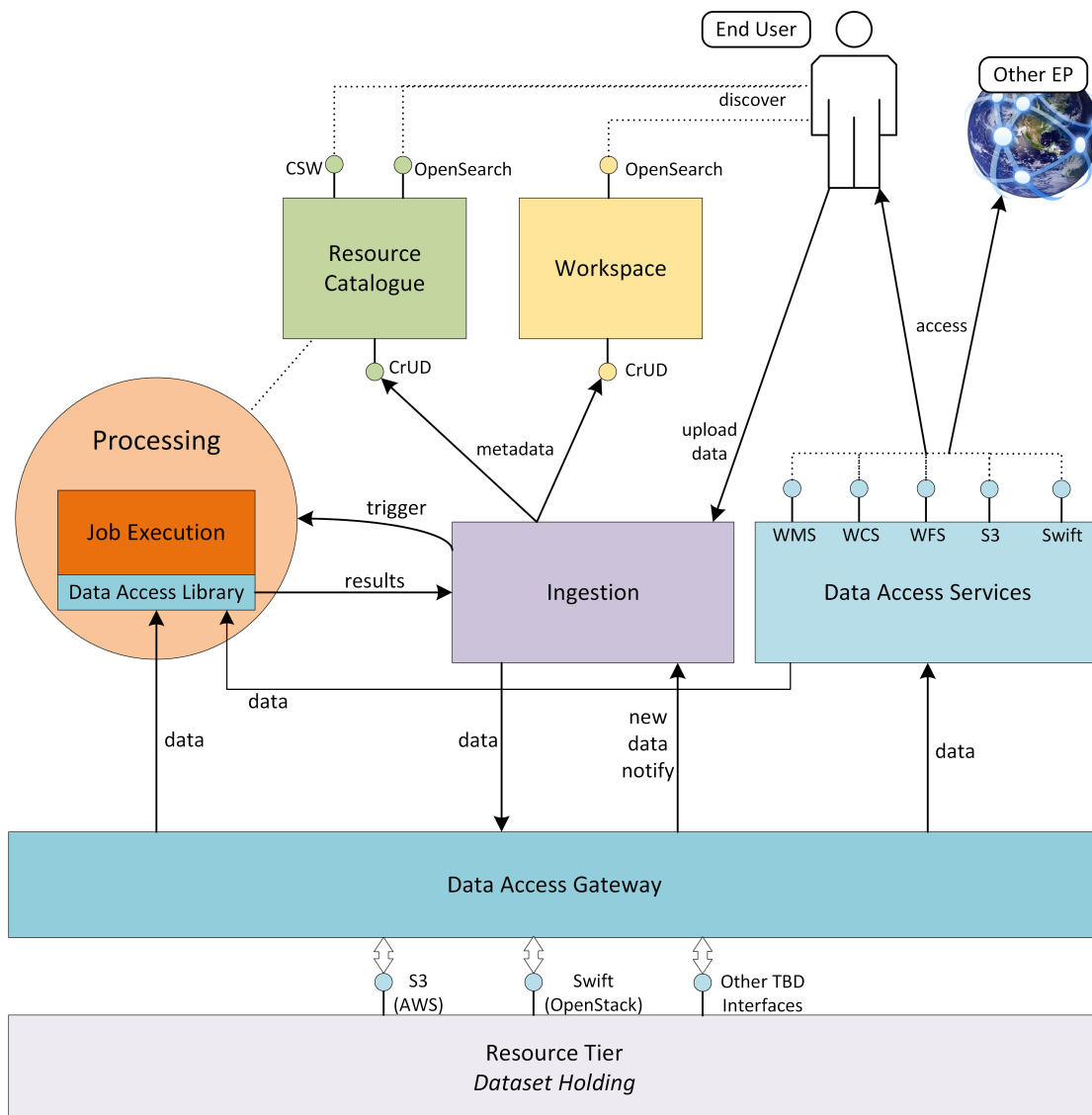
Figure 22. Resource Management Overview
