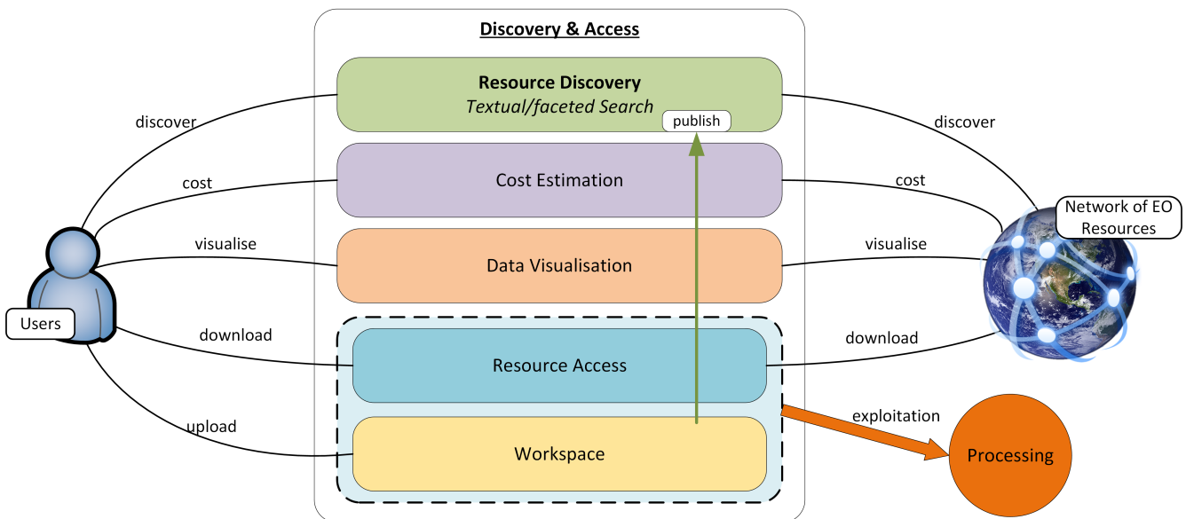
Figure 21. Resource Management Use Case
