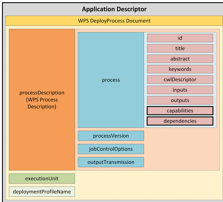
Figure 19. Application Descriptor (Enhanced)
