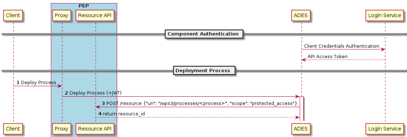
Figure 11. Dynamic Resource Registration through a Resource API
