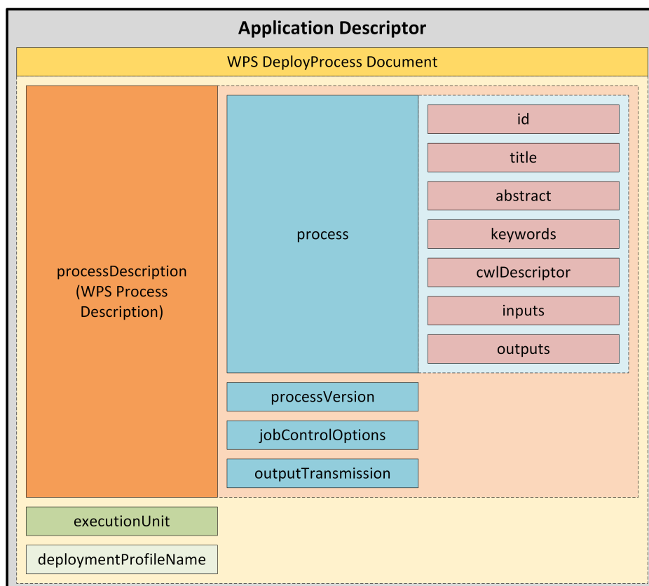
Figure 14. Structure of Application Descriptor data model
