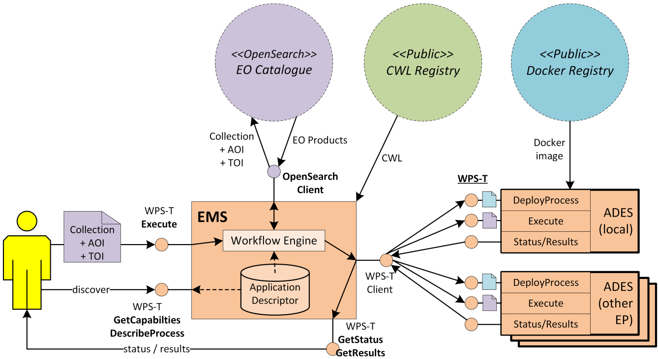
Figure 16. EMS Workflow Execution
