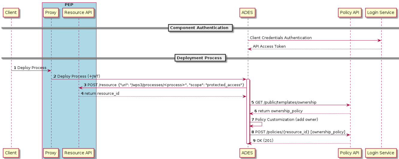
Figure 9. Dynamic Resource Protection through a Policy API
