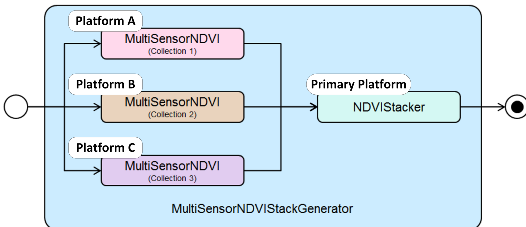
Figure 27. OGC Testbed-14 Workflow Scenario (NDVI Stacker)
