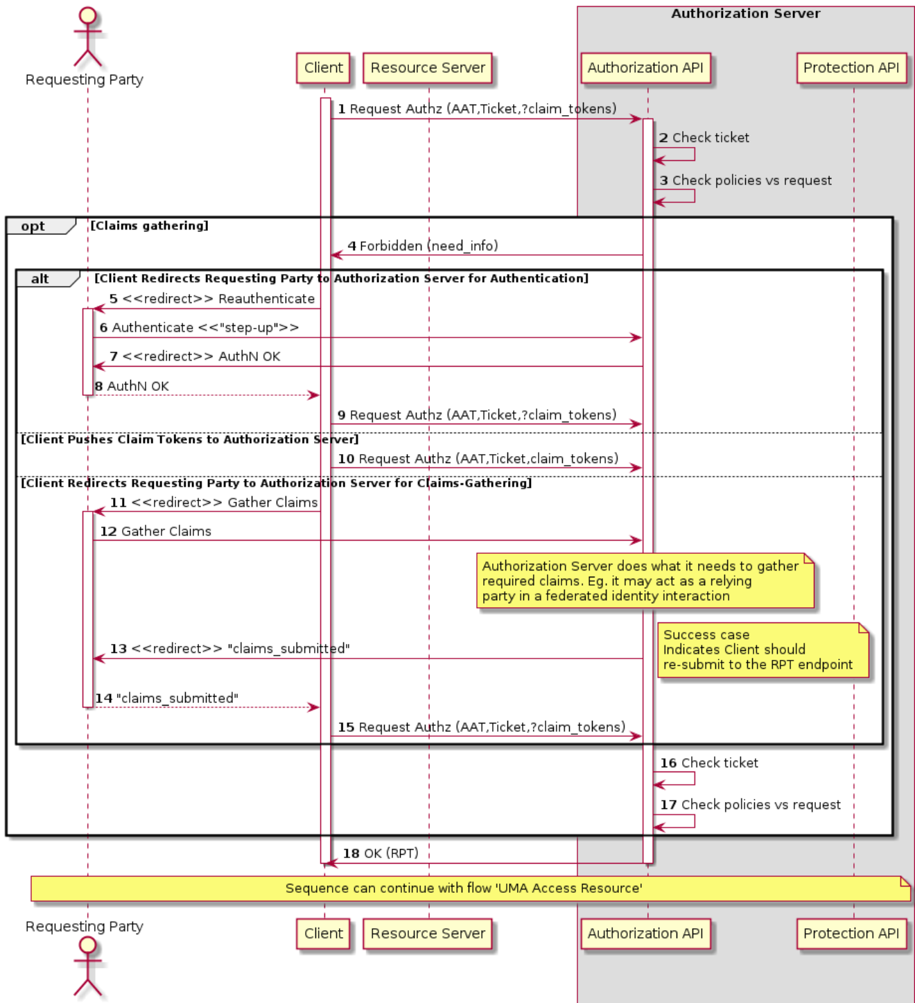
Figure 8. UMA Client Request Authorization
