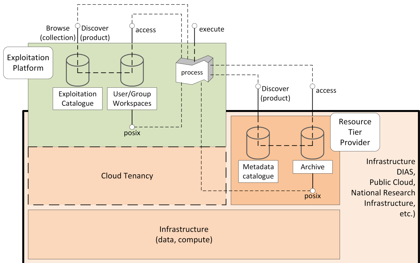
Figure 21. Catalogue Aggregation
