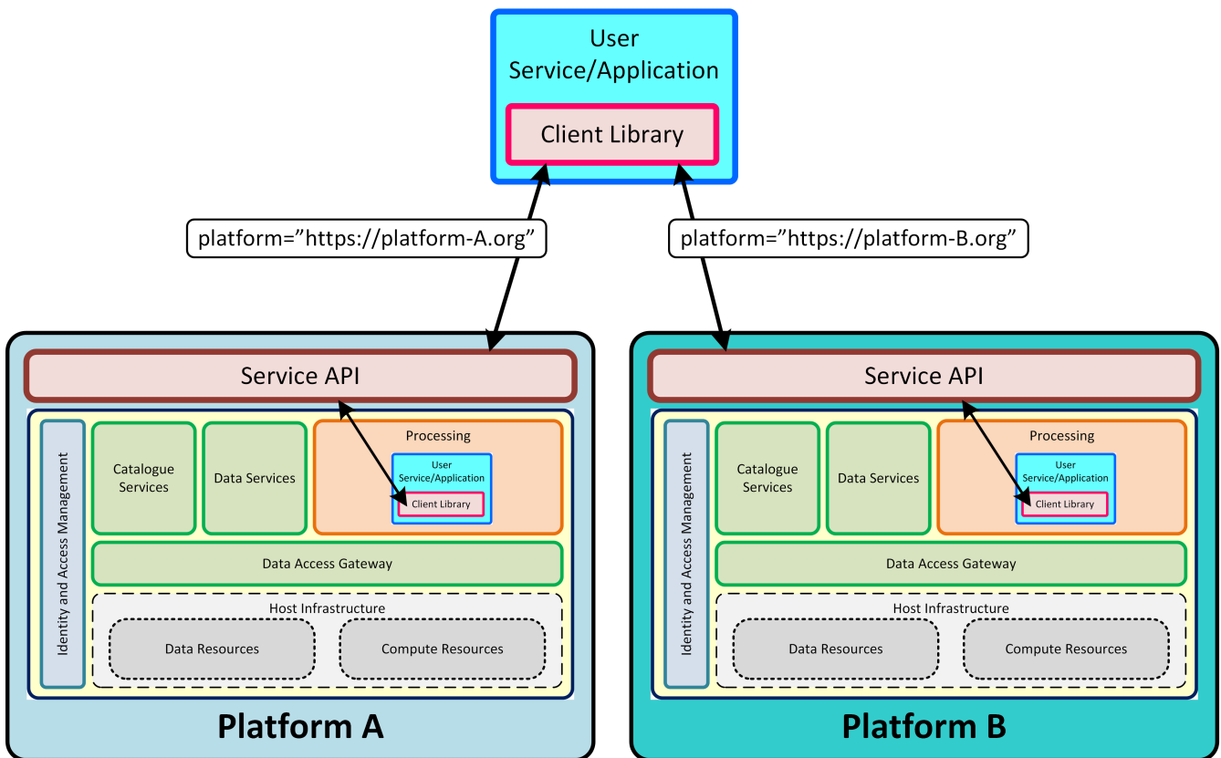
Figure 23. Client Portability
